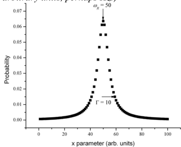
Figure 3: Lorentzian Distribution
