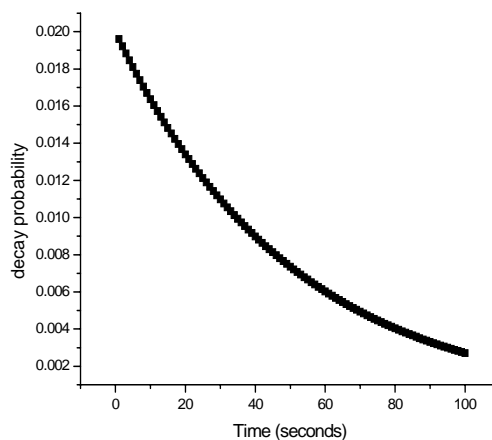
Figure 4 Exponential Decay
