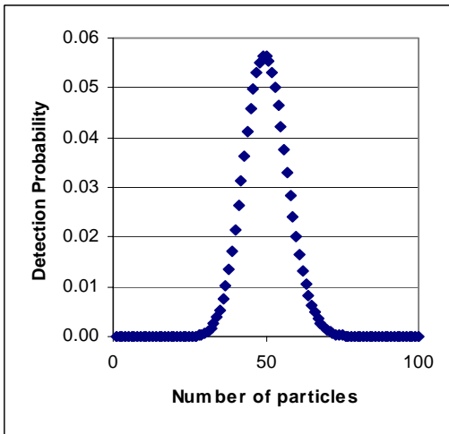
Figure 2: Poisson Distribution
